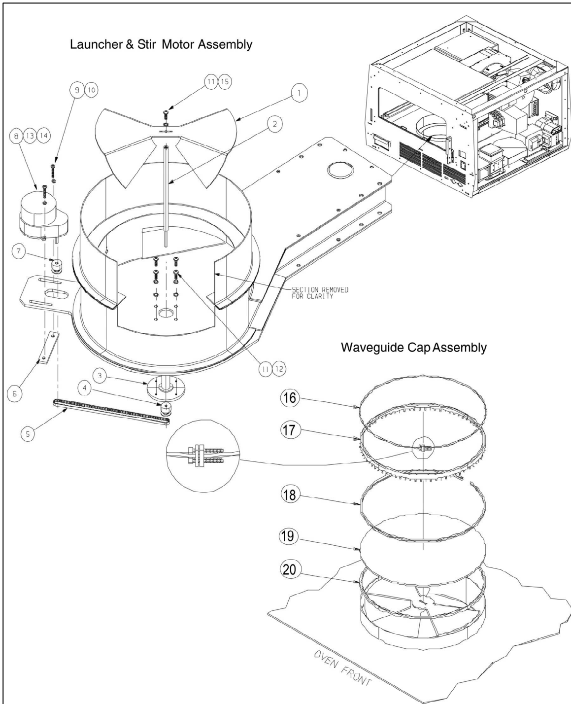
Figure 9-6: Waveguide Assy
